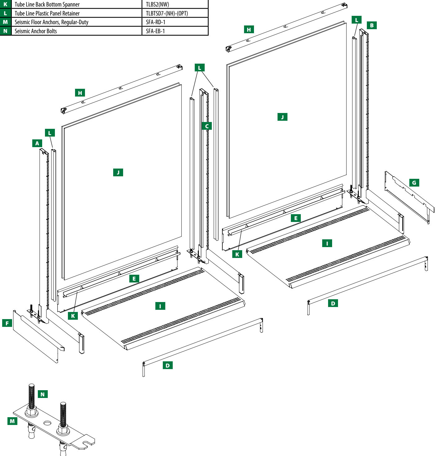
Enlargement of Seismic Floor Anchors & Bolts
