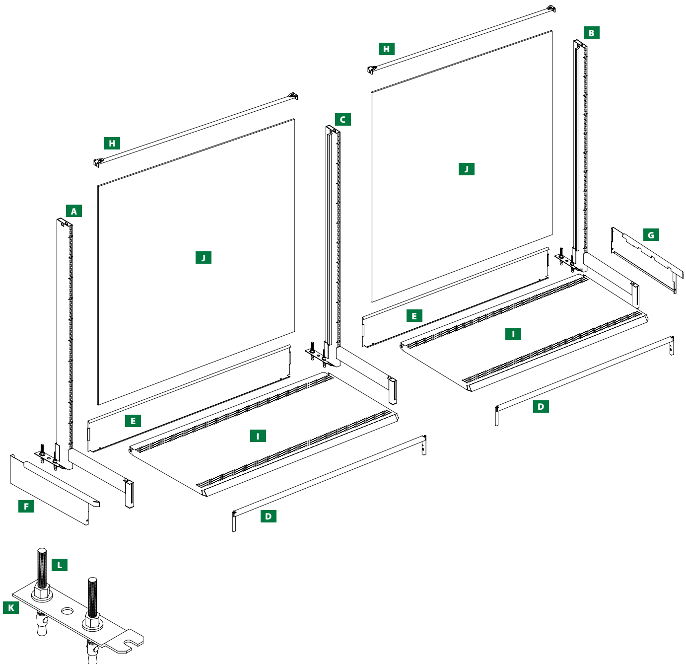
Enlargement of Seismic Floor Anchors & Bolts
