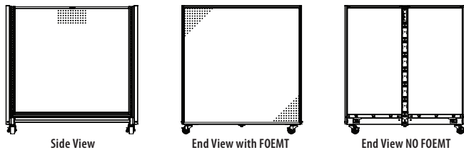
Basic Unit with Standard Base Shelf and TLRTAZ Tie Bars
