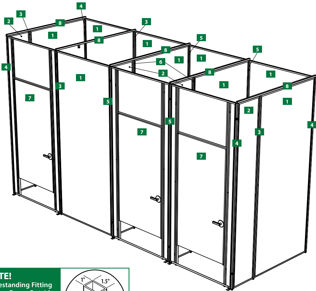
Tube Line Freestanding Three Bay Fitting Room consists of two standard rooms and one ADA room
