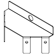
Outside Corner Detail
