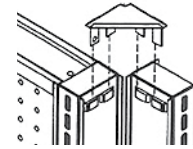
Outside Corner Detail
