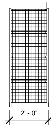
SIDE ELEVATION
